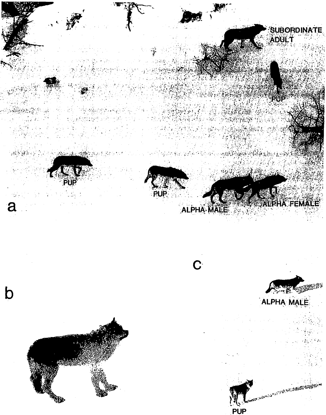
Figure 4. Isle Royale wolves, 1983. a) West Pack II, b) West Pack II pup, c) Harvey Lake Pack wolves.
