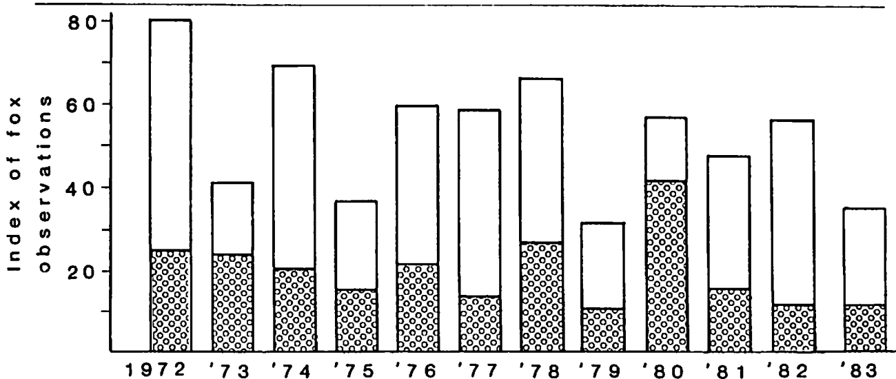
Figure 15. Midwinter fox index, 1972-83. The lower bar is the number of foxes seen > 1 km from a moose carcass/100 hrs flying time, while the upper bar is the sum of the maximum number of foxes seen on each moose carcass.
