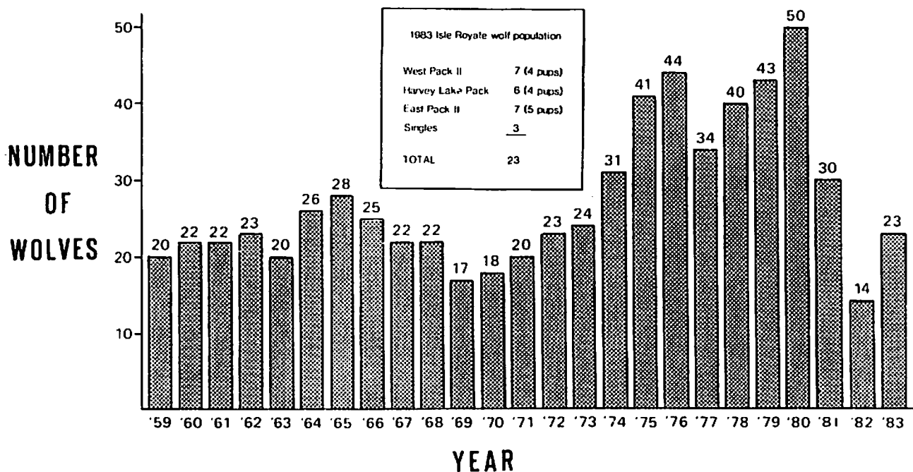
Figure 2. Isle Royale wolf population fluctuations, 1959-83.
