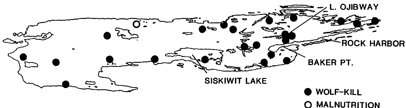
Figure 10. Distribution of all moose carcasses located during 1983 winter study, together with place names mentioned in text.
